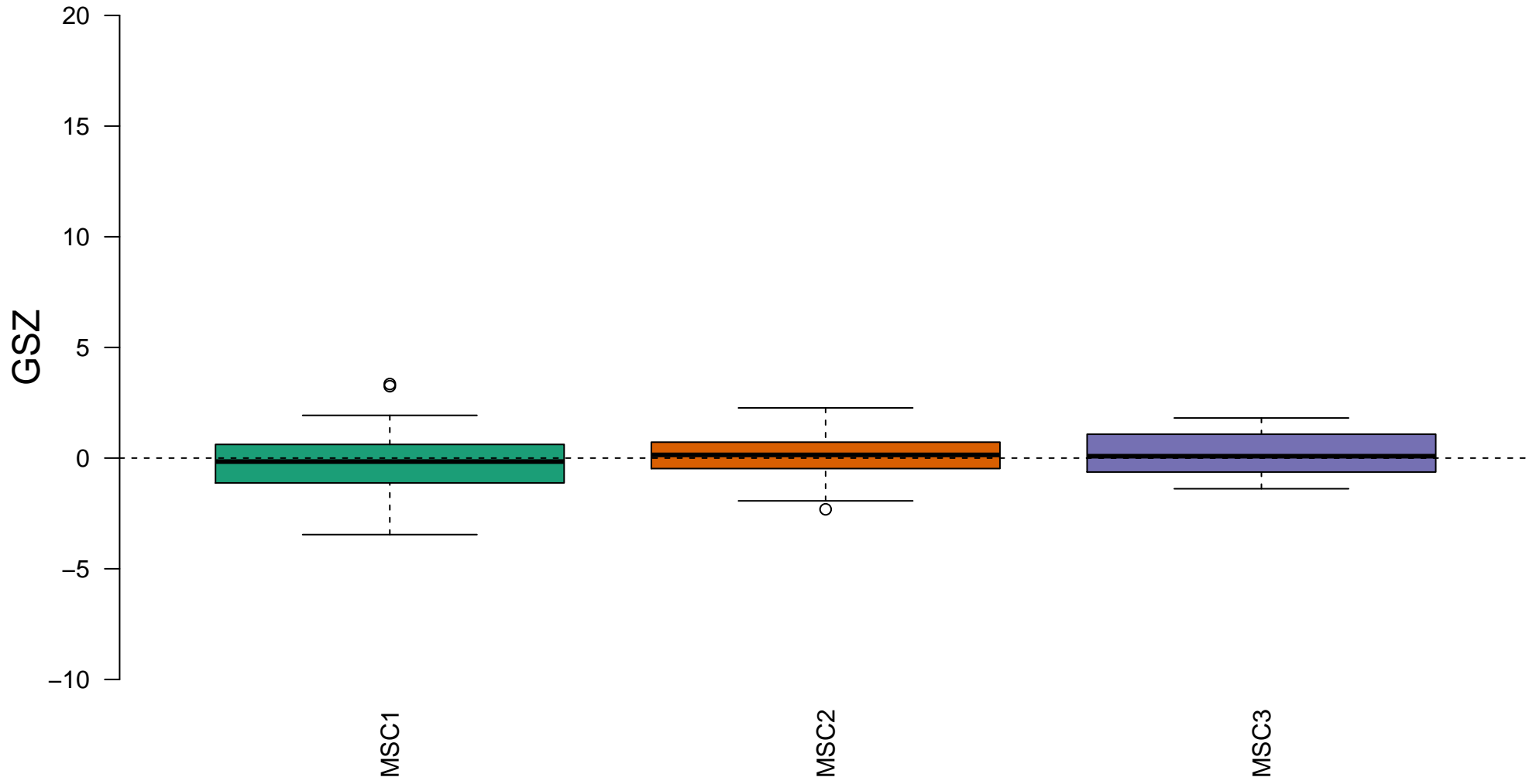
Pentrack_CRC_TCGA_corr_N_msi-h_DN
